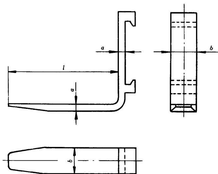
挂钩型货叉
